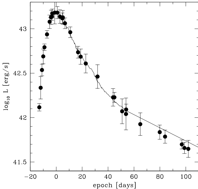
Figure 4. uvoir light curve of SN 2002bo. The solid line is the uvoir light curve of SN 1998bu reconstructed from the published UBVR data and adding the UV and IR contributions given in Suntzeff (1996) for a sample of SNIa. The error bars refer only to the photometric errors and not to the uncertainty related to the reddening.
